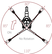
Microphone Boom Rotation
